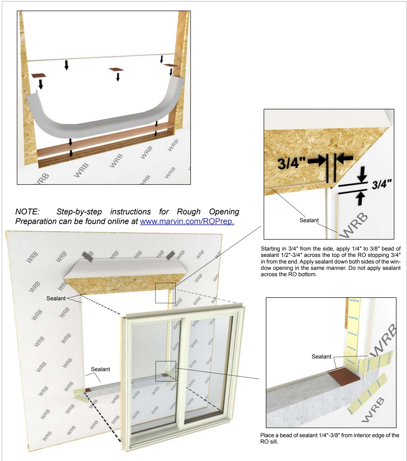
Figure 3 For step by step instructions on how to prepare an opening, refer to www.marvin.com/ROprep .
